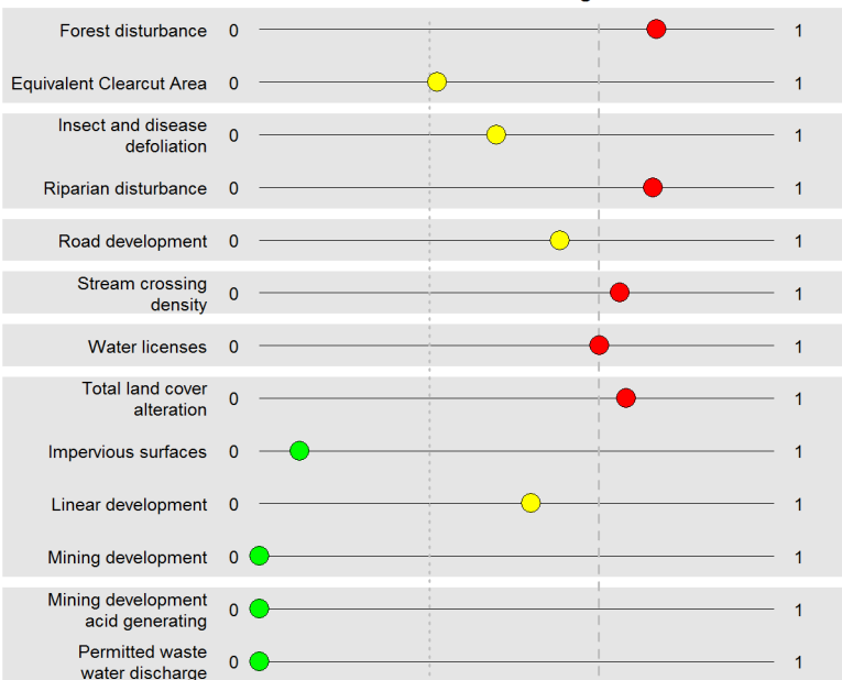
Area weighted average of all watershed scores (normalized) for McDonnell CU rearing lake ZOI
