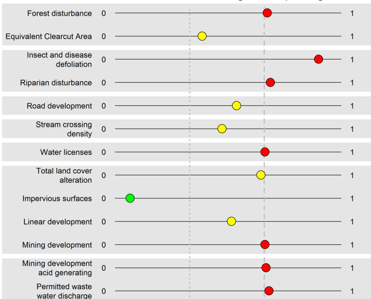
Area weighted average of all watershed scores (normalized) for Chinook Mid Skeena Large Lakes spawning ZOI
